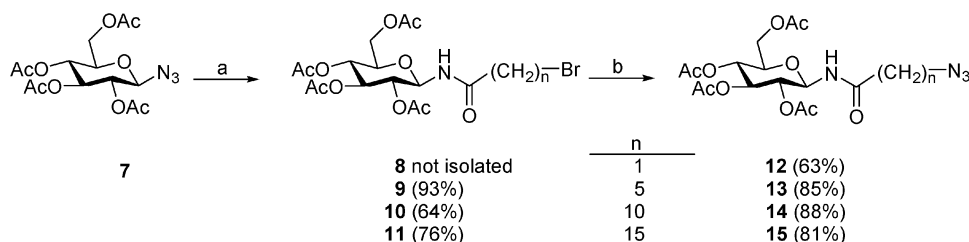
Scheme 2 Reagents and conditions: (a) PMe 3 , Br-(CH 2 ) n -COOH, CH 2 Cl 2 , rt; (b) NaN 3 , DMF, rt.
