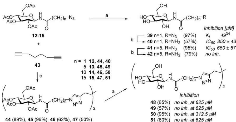
Scheme 5 Reagents and conditions: (a) cat. NaOMe, MeOH rt.; (b) RANEY ® -Ni, H 2 , MeOH, 70 °C; (c) CuSO 4 , L-ascorbic acid, CH 2 Cl 2 -H 2 O, rt. Inhibition of RMGPb.
