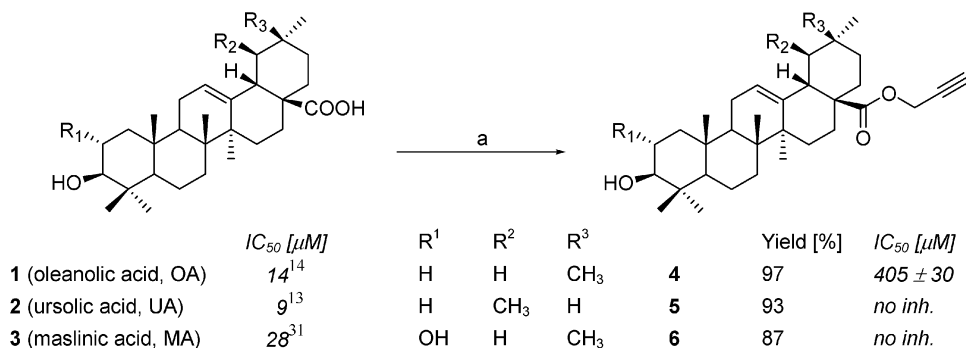
Scheme 1 Reagents and conditions: (a) K 2 CO 3 , propargyl bromide, DMF, rt. Inhibition of RMGPa ( IC 50 [μM], values are means of three experiments).
