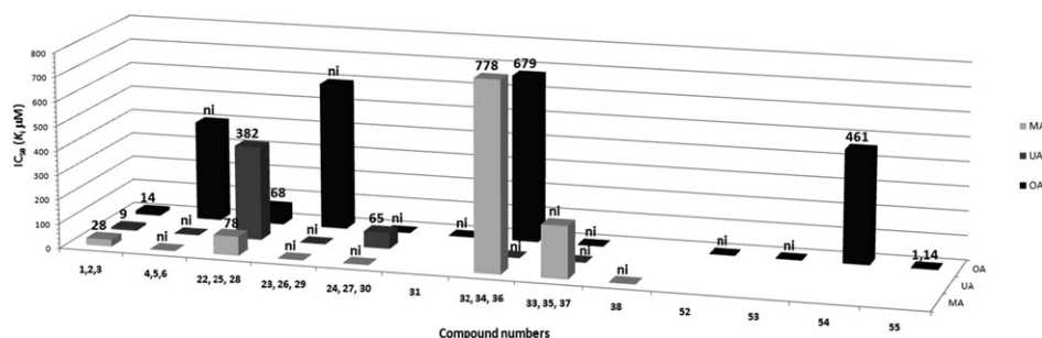
Chart 2 Comparison of inhibition assay results against RMGP a (abbreviations: derivatives of maslinic acid (MA), ursolic acid (UA) and oleanolic acid (OA); ni = no inhibition).
