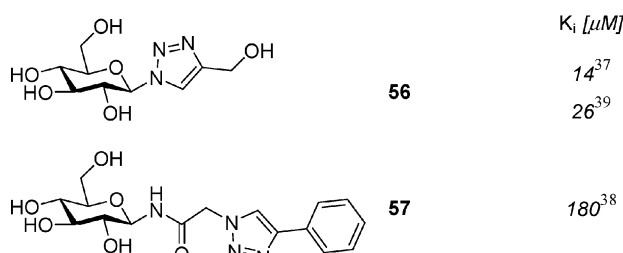
Chart 1 Literature data for some inhibitors of RMGP.
