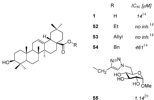
Scheme 5 Reagents and conditions: (a) cat. NaOMe, MeOH rt.; (b) RANEY ® -Ni, H 2 , MeOH, 70 °C; (c) CuSO 4 , L-ascorbic acid, CH 2 Cl 2 -H 2 O, rt. Inhibition of RMGPb.
